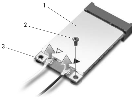
1 WLAN Card 2 M2 x 3-mm screw 3 antenna cable connectors (2)
